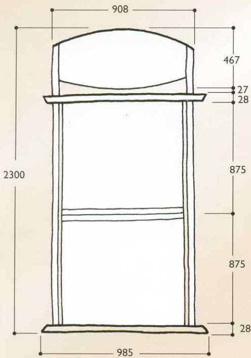
TWO UNITS WITH ROUNDED BOTTOMED HEADER
