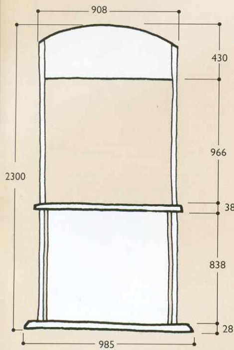
ONE UNIT WITH FLAT BOTTOMED HEADER
