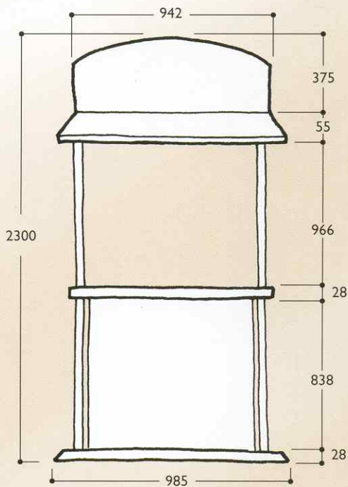
ONE UNIT WITH ROOF
