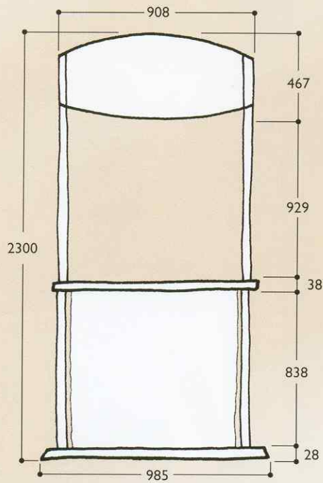
ONE UNIT WITH ROUNDED BOTTOMED HEADER
