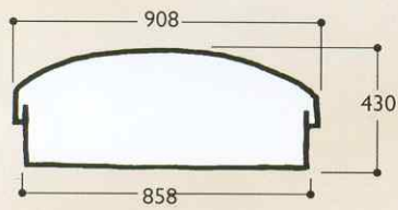
FLAT BOTTOMED HEADER
